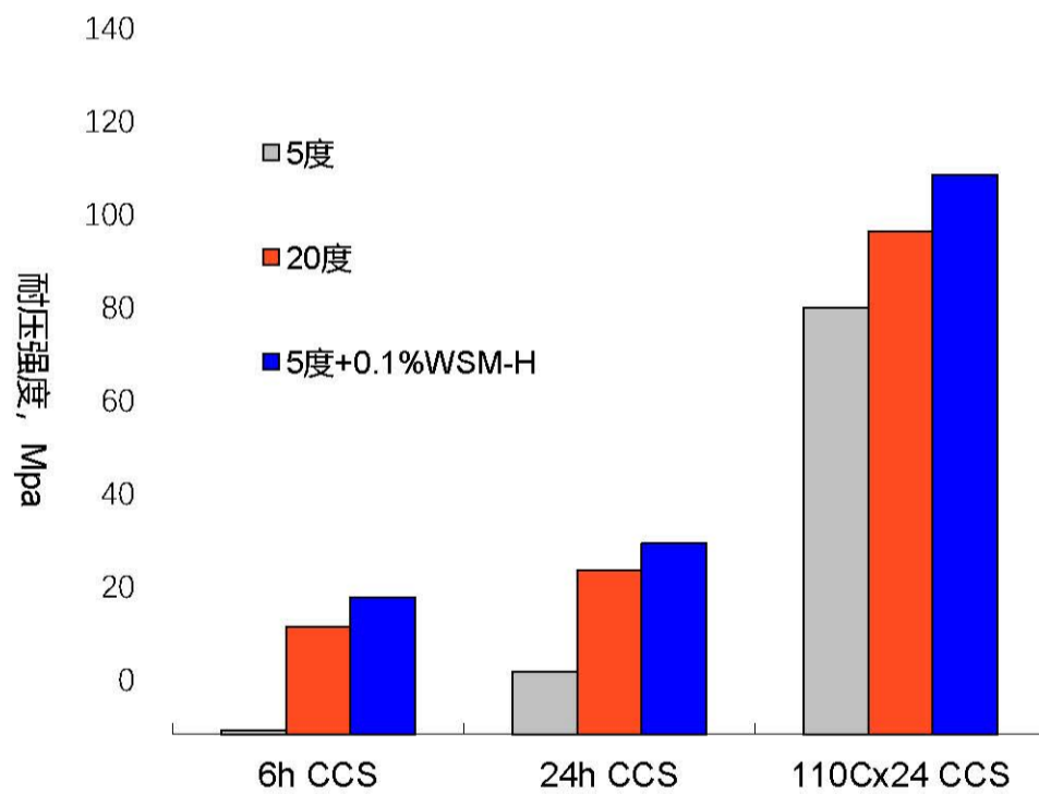
配方: 矾土骨料, 细粉: 5% Elkem971U; 5%S71
